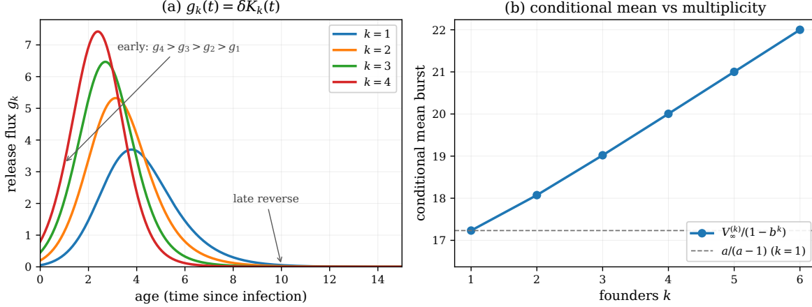
Figure 16: Multiplicity of infection at (\lambda, \mu, \delta) = (1, 0.2, 0.05) . (a) Release fluxes g_k(t) = \delta K_k(t) for k = 1, \dots, 4 : early ages are ordered superlinearly in founding load, while late fluxes reverse as multi-founder lineages fix faster. (b) Conditional mean burst V_\infty^{(k)}/(1 - b^k) increases with k ; the dashed line is the k = 1 value a/(a - 1) .
