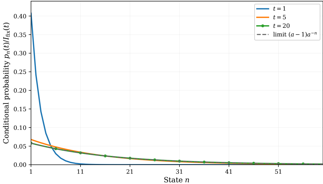
Figure 6: Conditional state probabilities p_n(t)/I_{\text{fix}}(t) converging to the geometric quasi-stationary law (a - 1)a^{-n} for (\lambda, \mu, \delta) = (1, 0.2, 0.05) . By t = 20 , the conditional mass function is visually indistinguishable from the dashed limit.
