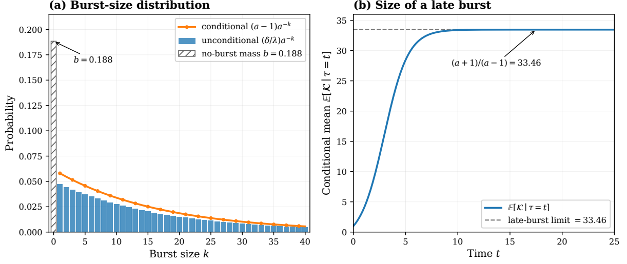
Figure 9: Burst-size and late-burst laws for (\lambda, \mu, \delta) = (1, 0.2, 0.05) . (a) The unconditional law (\delta/\lambda)a^{-k} , including the no-burst mass b at k = 0 , and the law (a - 1)a^{-k} conditioned on bursting. (b) The size-biased mean \mathbb{E}(\mathcal{K} \mid \tau = t) rises towards (a + 1)/(a - 1) = 33.46 .
