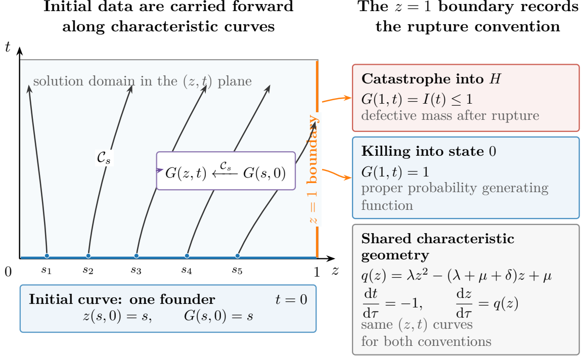
Figure 2: Method of characteristics for the single-cell probability generating function. The initial data z(s, 0) = s and G(s, 0) = s are carried along curves generated by dt/d\tau = -1 and dz/d\tau = q(z) , where q(z) = \lambda z^2 - (\lambda + \mu + \delta)z + \mu . The condition at z = 1 supplies the rupture bookkeeping: G(1, t) = I(t) under catastrophe, whereas G(1, t) = 1 when rupture is counted in state 0. Thus the solution is fixed by characteristic transport and the stated data rather than by a guessed ansatz.
