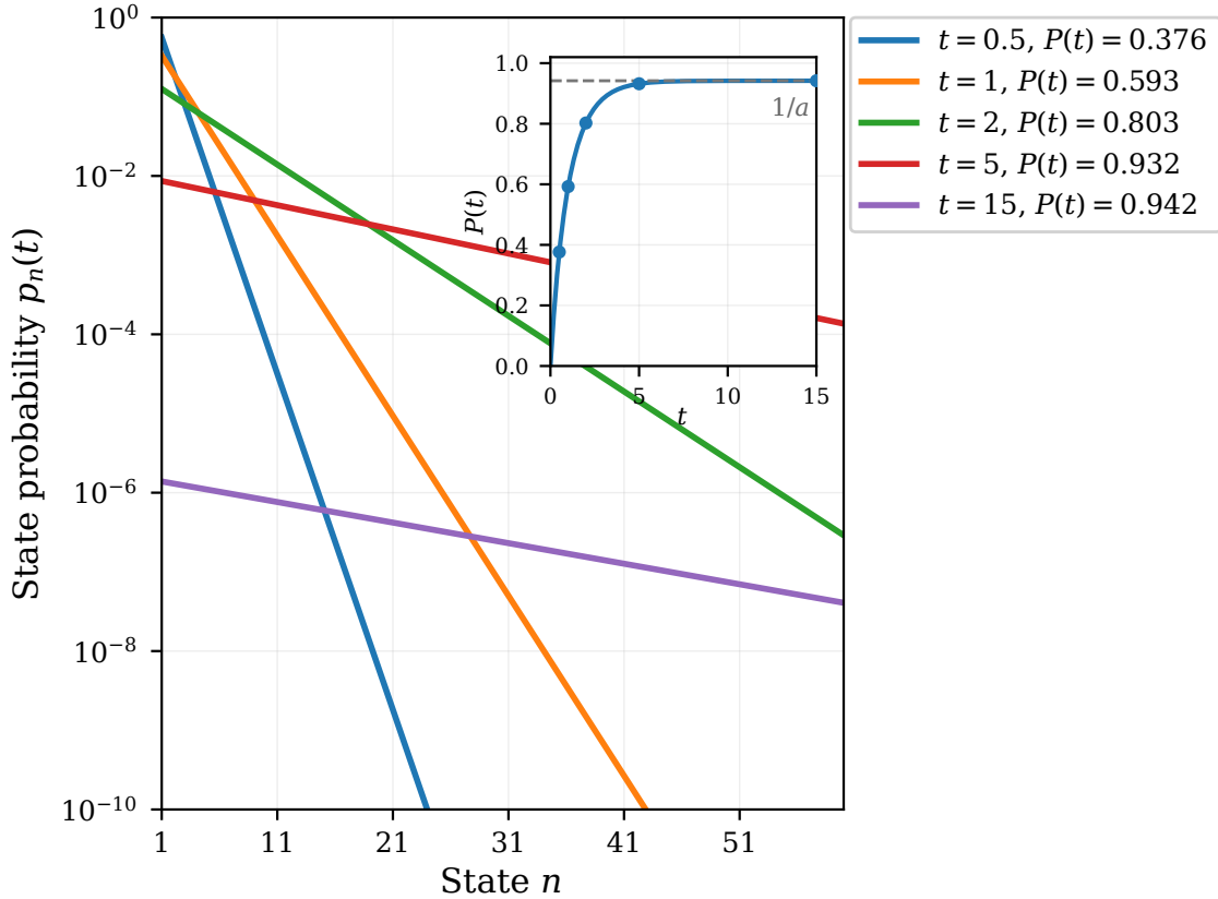
Figure 3: State probabilities p_n(t) at successive times for (\lambda, \mu, \delta) = (1, 0.2, 0.05) . On the logarithmic vertical scale, each geometric law is a straight line whose ratio P(t) increases towards 1/a ; the inset shows this approach directly.
