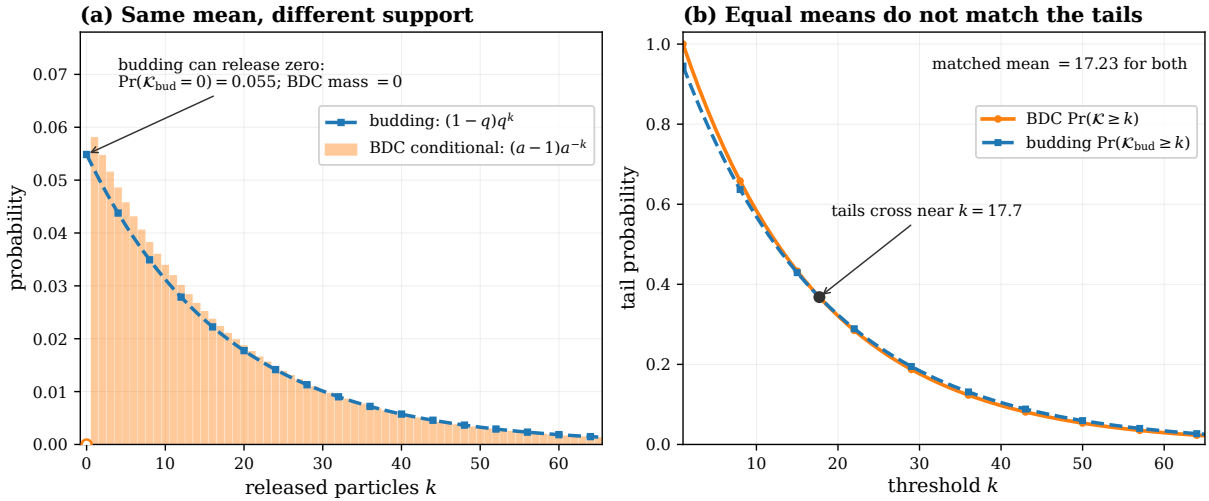
Figure 11: Release-count laws for the BDC process at (\lambda, \mu, \delta) = (1, 0.2, 0.05) and a budding comparator. The budding mean p/d_{\mathcal{I}} is matched to the BDC conditional mean V_{\infty}/(1 - b) = 17.23 . The BDC law conditioned on bursting is geometric on \{1, 2, \dots\} , whereas the budding law is geometric on \{0, 1, 2, \dots\} and retains probability 0.055 of zero release. Thus matching the means neither matches the support nor the tails.
