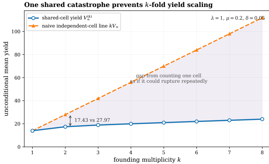
Figure 15: Unconditional mean yield V_\infty^{(k)} against founding multiplicity k , compared with the naive independent-cell line kV_\infty , for (\lambda, \mu, \delta) = (1, 0.2, 0.05) . The true yield is sub-extensive because all founders share one cell and hence one catastrophe; for k = 2 , V_\infty^{(2)} = 17.43 , rather than 2V_\infty = 27.97 .
