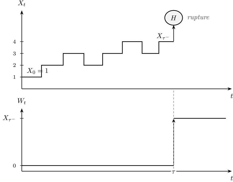
Figure 1: A representative path of the joint process (X_t, W_t) . The intracellular load follows a birth–death path until rupture at time \tau , when X_t enters the absorbing state H . At the same instant, the released count jumps from zero to the pre-rupture load X_{\tau-} and remains there.
