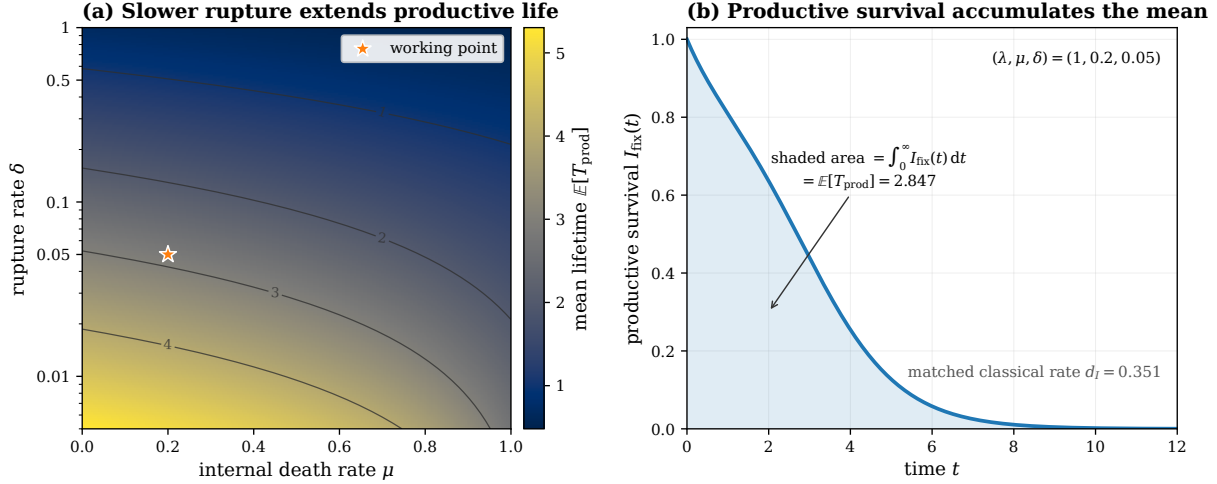
Figure 7: Mean productive lifetime \mathbb{E}(T_{\text{prod}}) = \lambda^{-1} \log(a/(a-1)) . (a) Its dependence on \mu \in [0, 1] and \delta \in [0.005, 1] at \lambda = 1 ; contours give lifetime values and the star marks the working point. (b) The productive-survival curve I_{\text{fix}}(t) at (\lambda, \mu, \delta) = (1, 0.2, 0.05) , with its integral \mathbb{E}(T_{\text{prod}}) = 2.847 shaded. The corresponding matched classical death rate for Chapter 4b is d_I = 1/\mathbb{E}(T_{\text{prod}}) = 0.351 .
