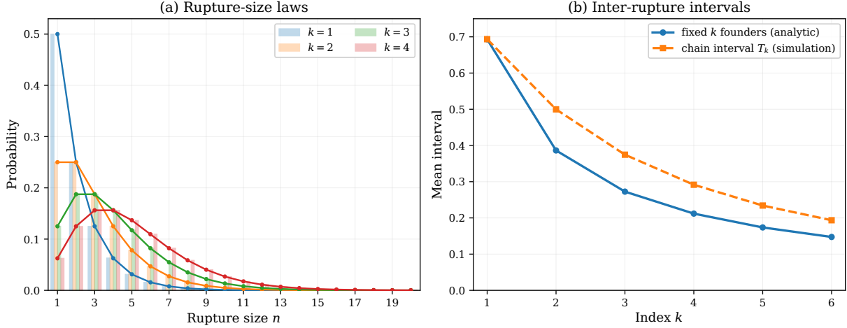
Figure 17: Chained immediate transfer with (\lambda, \delta) = (1, 1) and s = \rho = 1/2 . (a) Simulated rupture-size probabilities (bars) from 10^6 chain realisations with seed 42, together with the exact negative-binomial laws (connected curves) for k = 1, \dots, 4 . (b) The analytic mean interval for a fixed founding load k and the simulated mean interval at chain position k ; both decrease over k = 1, \dots, 6 .
