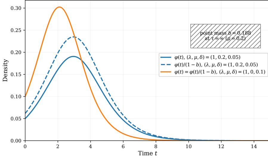
Figure 8: Defective burst-time density \varphi(t) = \delta J(t) and its conditional counterpart \varphi(t)/(1-b) . For (\lambda, \mu, \delta) = (1, 0.2, 0.05) , the finite-time density has total mass 1-b and the remaining mass b = 0.188 lies at \tau = \infty ; for (1, 0, 0.1) , b = 0 and the defective and conditional densities coincide.
