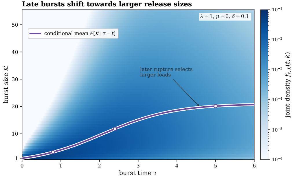
Figure 10: Joint density (with respect to time and counting measure) of burst time \tau and burst size \mathcal{K} for (\lambda, \mu, \delta) = (1, 0, 0.1) . The analytic overlay is the conditional mean \mathbb{E}(\mathcal{K} \mid \tau = t) = K(t)/J(t) , which rises from 1 towards 21. The upward tilt makes the geometric content of size-biasing explicit: later bursts preferentially occur from larger loads.
