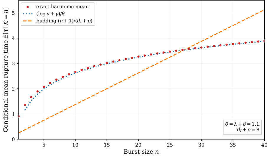
Figure 12: Conditional mean rupture time given burst size n when \mu = 0 , with \lambda = 1 , \delta = 0.1 , and hence \theta = 1.1 . Exact harmonic means \theta^{-1}H_n are shown with the large- n approximation \theta^{-1}(\log n + \gamma) and the linear budding comparator (n + 1)/(d_{\mathcal{I}} + p) at d_{\mathcal{I}} + p = 8 .
