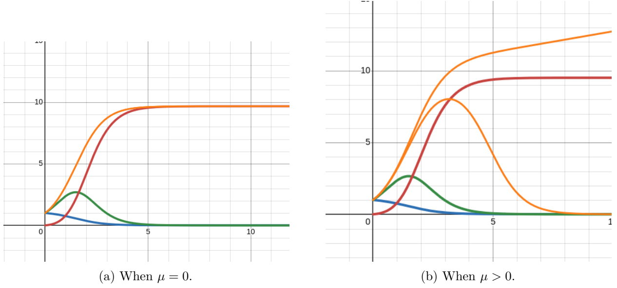
Figure 5: Conditional means from simulation. (a) When \mu = 0 , the conditional mean J(t)/I(t) tends to the same limit as V(t) , namely 1 + \lambda/\delta . (b) When \mu > 0 , the curve rising at late time is the mean conditioned on non-fixation, J(t)/I_{\text{fix}}(t) , tending to \langle X \rangle_{\text{QS}} = a/(a - 1) ; the curve tending to 0 is the mean conditioned only on non-catastrophe, \mathbb{E}(\mathbf{X}_t | \mathbf{X}_t \neq H) = J(t)/I(t) , which vanishes because a fraction b of realisations die out internally.
