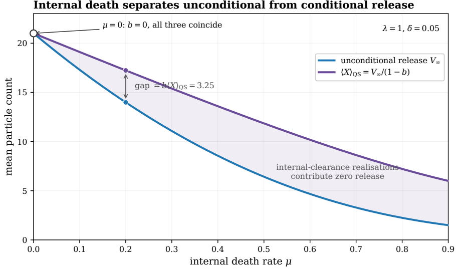
Figure 4: Quasi-stationary and release means across internal death rates at \lambda = 1 and \delta = 0.05 . The quasi-stationary mean \langle X \rangle_{\text{QS}} = a/(a-1) is identically the conditional burst mean V_\infty/(1-b) . At \mu = 0 , b = 0 and both also equal V_\infty ; once \mu > 0 , internally cleared cells contribute zero release and place V_\infty strictly below the other two quantities.
