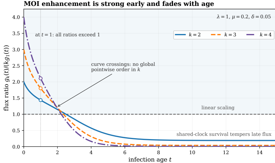
Figure 14: Release-flux ratios g_k(t)/(kg_1(t)) for k = 2, 3, 4 at (\lambda, \mu, \delta) = (1, 0.2, 0.05) . Values above 1 mark superlinear release relative to k independent single-founder cells. All three ratios are superlinear early, but their crossings and subsequent decay show that the enhancement is age-dependent rather than a pointwise ordering valid for all t .
