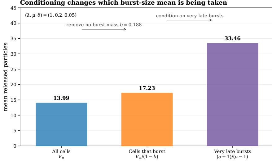
Figure 13: Three distinct averages at (\lambda, \mu, \delta) = (1, 0.2, 0.05) . The unconditional mean release V_\infty = 13.99 includes cells that never burst; conditioning on eventual burst gives V_\infty/(1-b) = a/(a-1) = 17.23 ; conditioning on a very late eventual burst gives the size-biased limit (a+1)/(a-1) = 33.46 . Keeping the conditioning explicit removes the apparent circularity.
